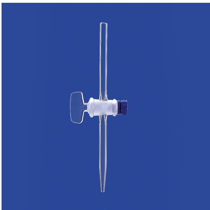
Burette stopcock, straight, with glass plug
