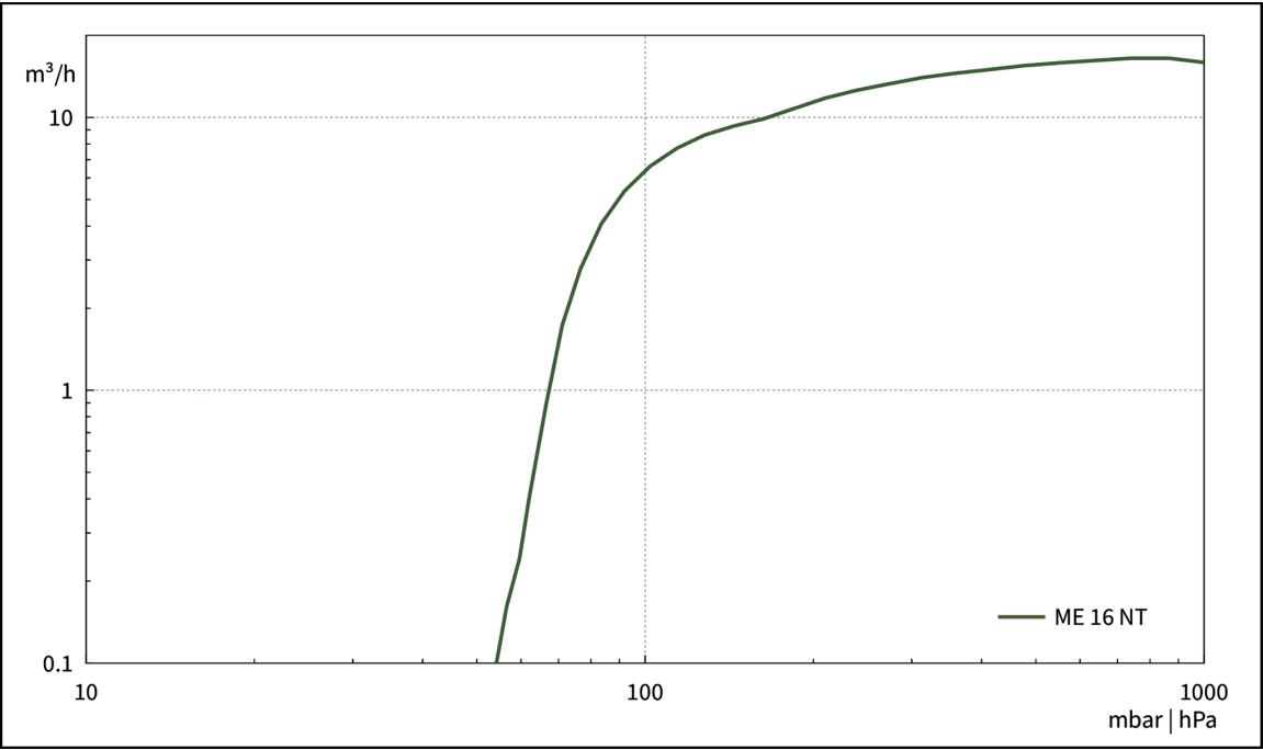
Pump down graph at 50 Hz (100 l volume)
