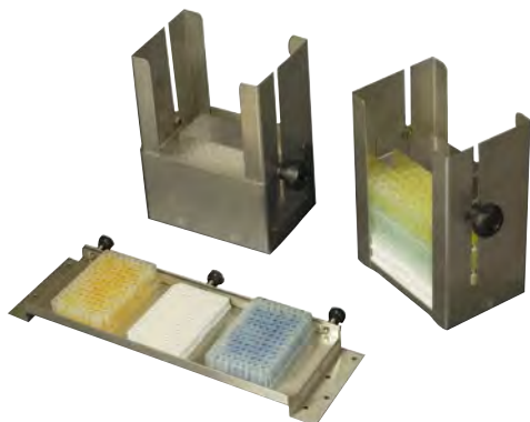
Microplate racks
